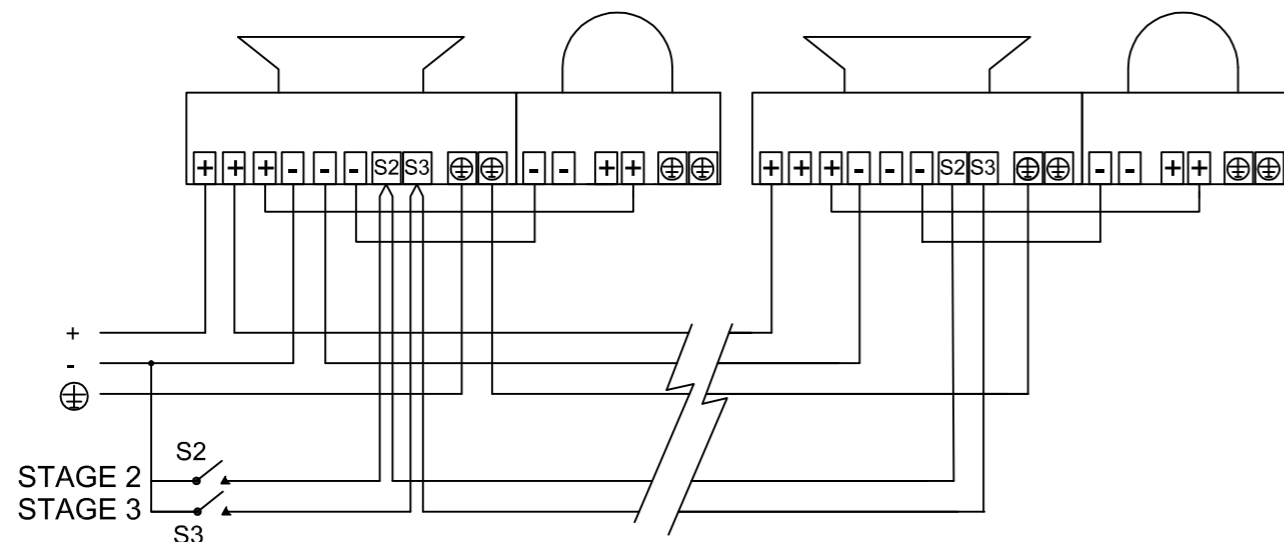
D2xC2XH1 / D2xC2XH2 - SIMULTANEOUSLY POWERED SOUNDER & BEACON
