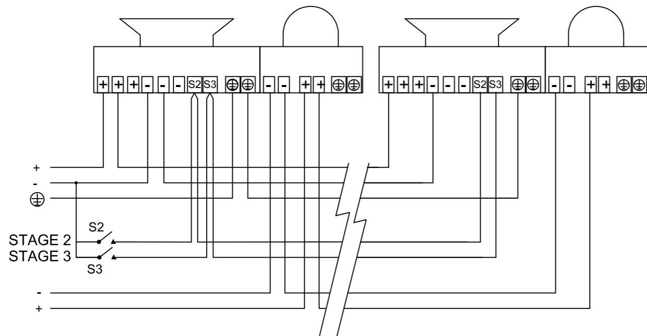
D2xC2XH1 / D2xC2XH2 - INDEPENDENTLY POWERED SOUNDER & BEACON
