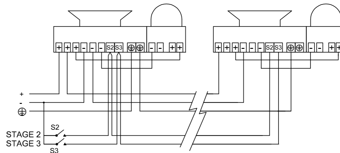
D2xC2LD3 - SIMULTANEOUSLY POWERED SOUNDER & BEACON
