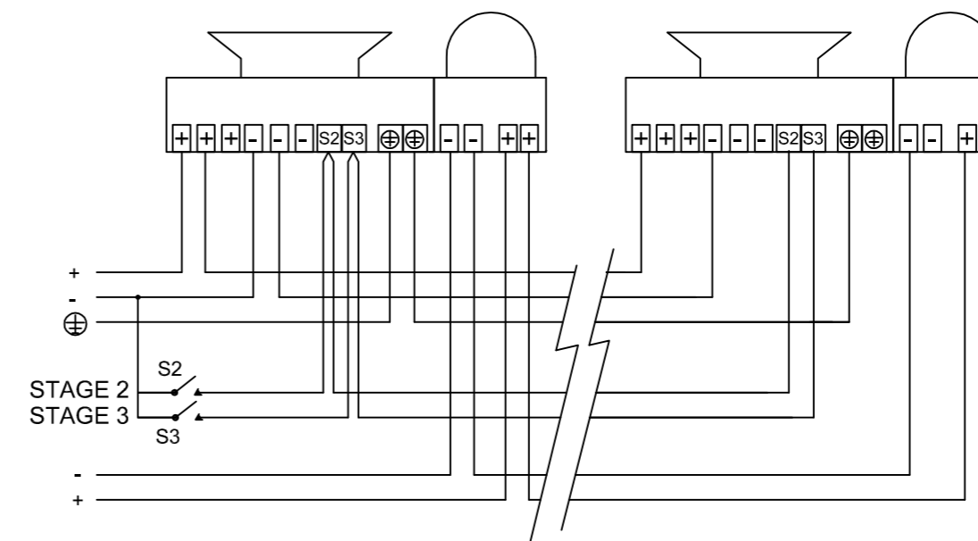
D2xC2LD3 - INDEPENDENTLY POWERED SOUNDER & BEACON
