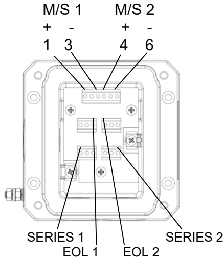
Fig. 5 PCB Terminal Block in Base
