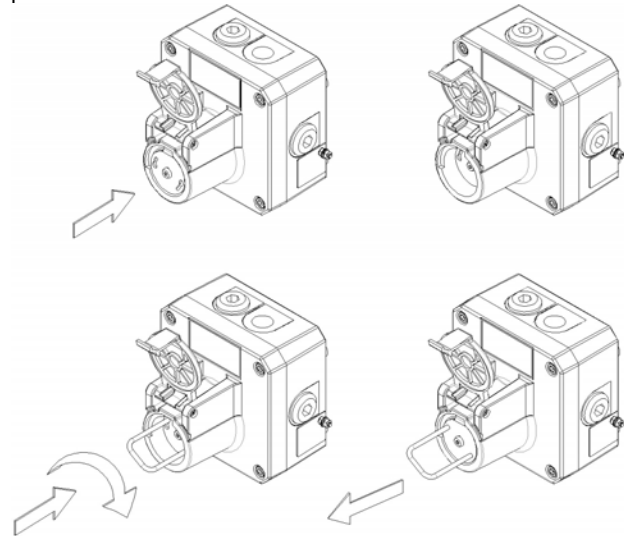
Fig 8a -PT Version Push Action
