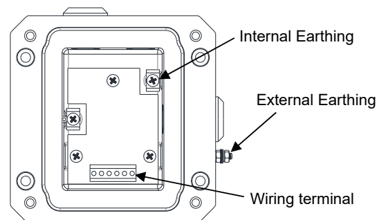
Fig 3 Earth terminals
