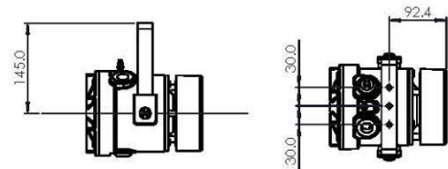
Fig. 1c Fixing Locations for Radial Horn
