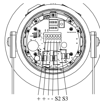
Fig. 6 DC Terminals
