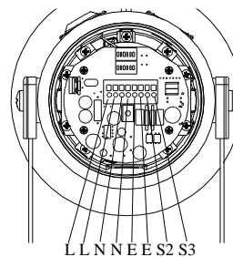
STExS1AC Terminals
