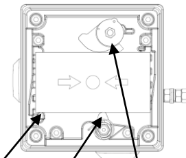
Pivot point Test Cam Top Cam (rotate)
