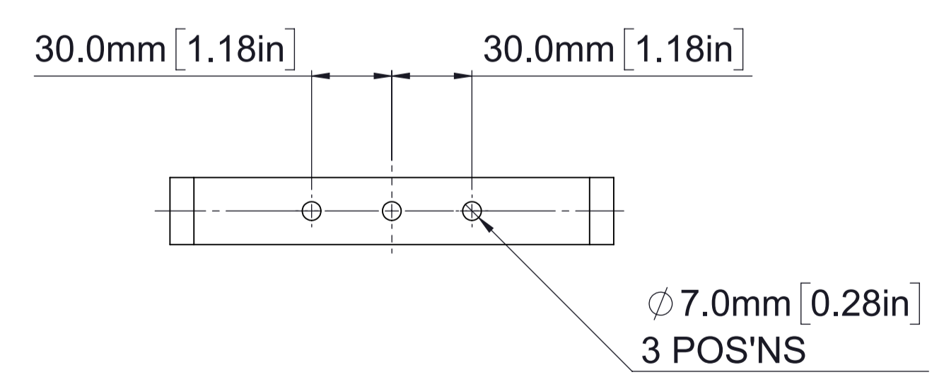
SCRAP VIEW IN DIRECTION 'A'
